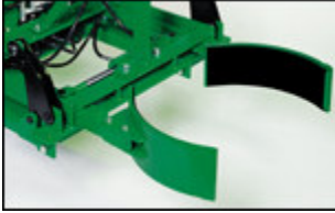
Standard Jaws for steel drums and cylinders 8-28 in. in diameter.
