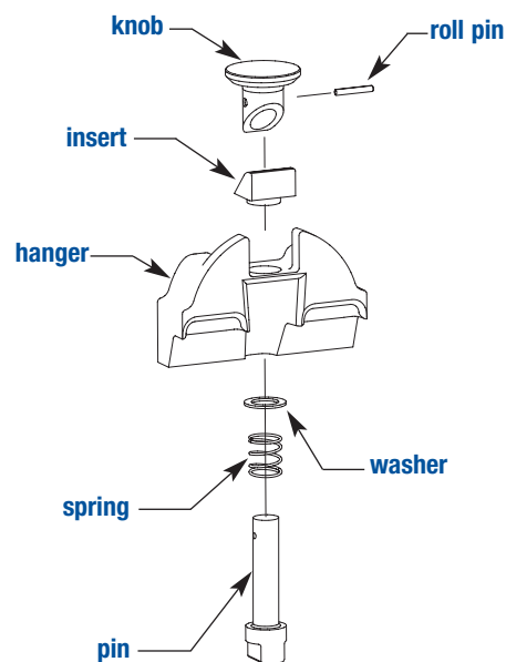
retro fit assembly
